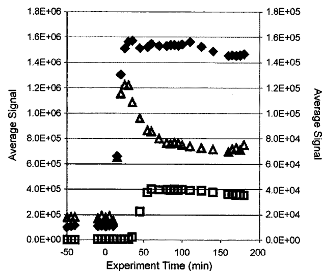
Fig. 6. Reaction time profiles of T → F pairs m/z 139 → 121 (♦, left axis), m/z 157 → 121 (Δ, right axis) and m/z 157 → 111 (□, left axis) showing the delayed formation of the unique product at target m/z 157 using T → F pair 157 → 111.
