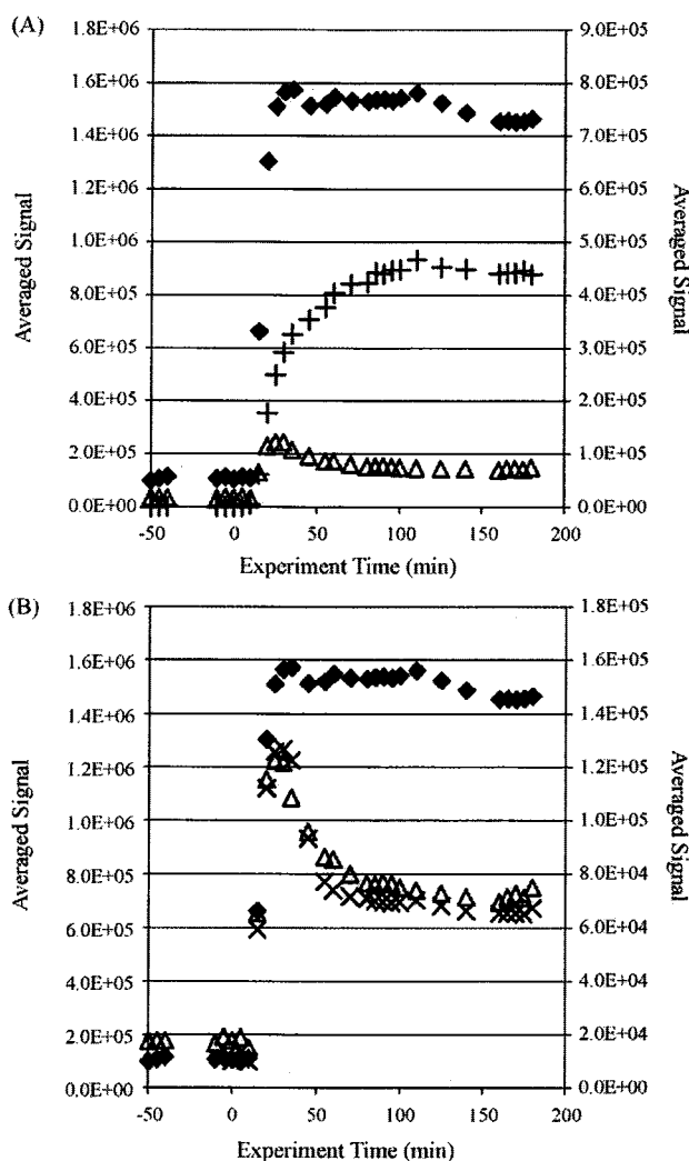
Fig. 9. Reaction time profiles of (A) T \rightarrow F pairs m/z 139 \rightarrow 121 ( \blacklozenge , left axis), m/z 157 \rightarrow 121 ( \triangle , right axis) and m/z 197 \rightarrow 121 (+, right axis) and (B) T \rightarrow F pairs m/z 139 \rightarrow 121 ( \blacklozenge , left axis), m/z 139 \rightarrow 121 subtract m/z 157 \rightarrow 111 and m/z 197 \rightarrow 121 ( \times , left axis) and m/z 157 \rightarrow 121 ( \triangle , right axis).
