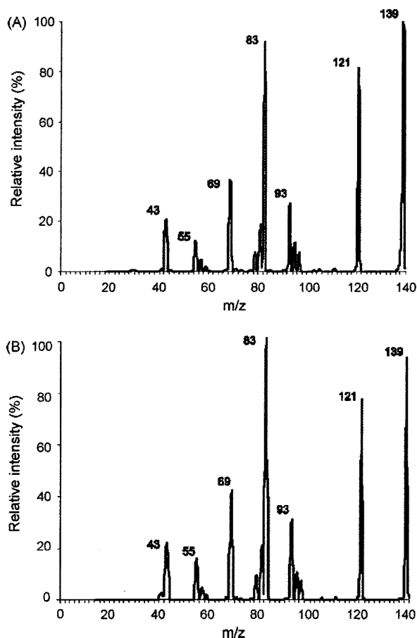
Fig. 2. Comparison of the MS/MS spectra of target m/z 139 from (A) the reaction mixture and (B) a pinaketone standard sample. The collision energy for both samples is 10 eV.
