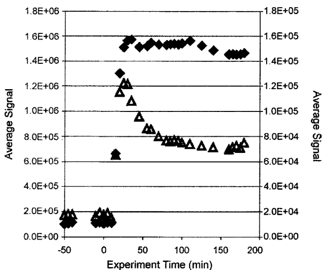
Fig. 4. Reaction time profiles of T → F pairs 139 → 121 (♦, left axis) and m/z 157 → 121 (Δ, right axis) of pinaketone. The 157 → 121 profile shows the expected profile of pinaketone with decay due to reactivity to HO radicals. The 139 → 121 pair is proposed to have contributions from products in addition to pinaketone, see text.
